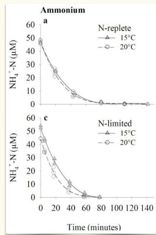
Depletion curves obtained from a perturbation experiment
