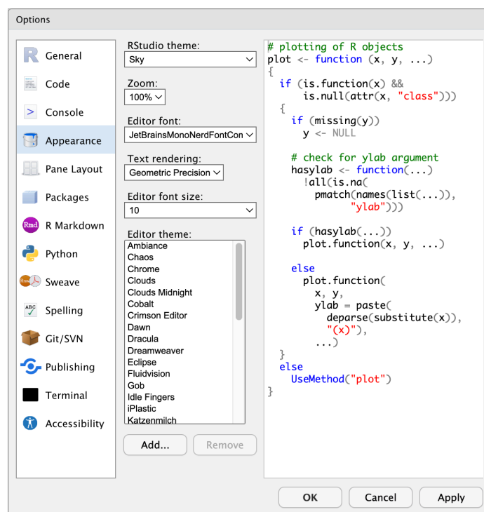
Figure 4: Appearance settings
