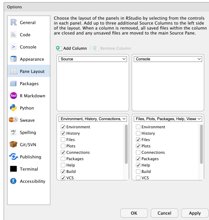
Figure 5: Rearranging the panes
