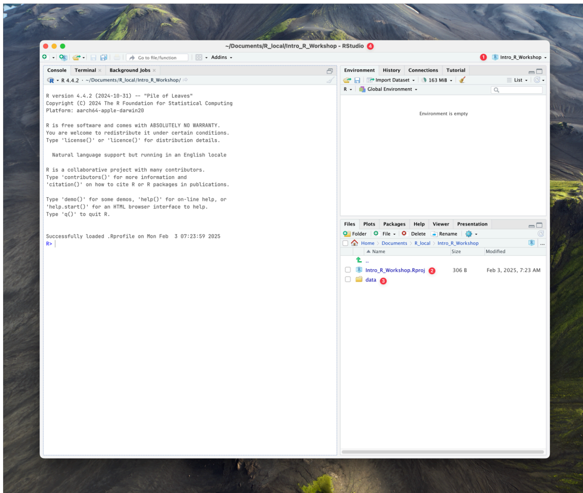
Figure 6: RStudio project
