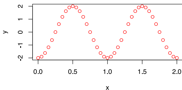
Figure 7: A plot assembled with the base R plot function.
