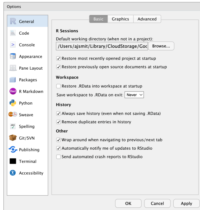
Figure 3: RStudio preferences
